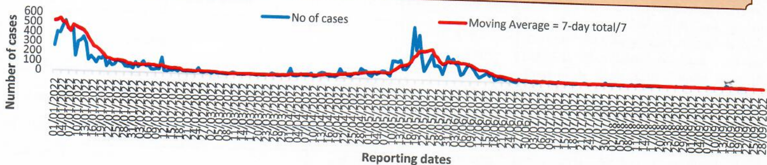
Figure 2: The 7 days moving average line chart for confirmed COVID-19 cases, 28 September 2022
